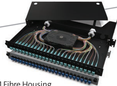
Everon LAN1 Fibre Housing Up to 96 fibres
